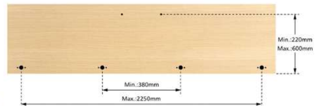
MB2041 drill style
